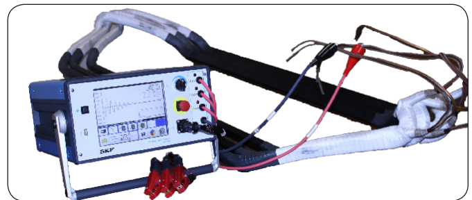
Testing a coil utilizing the Baker DX.
