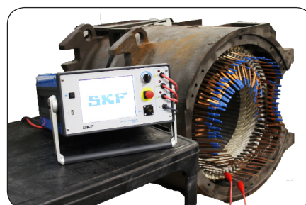
Testing individual coils within the stator.
